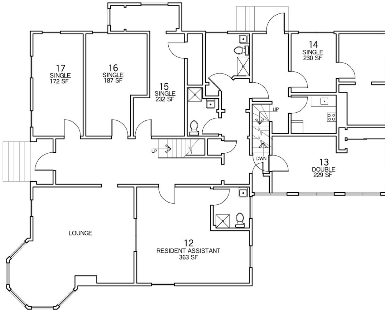
Barstow House 62 Waterman Street First Floor Plan
