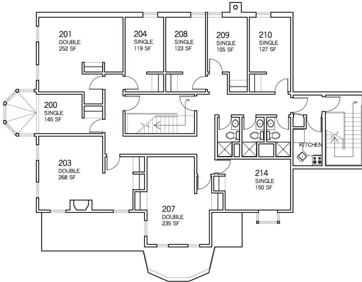
Dexter House 187 Benefit Street Second Floor Plan
