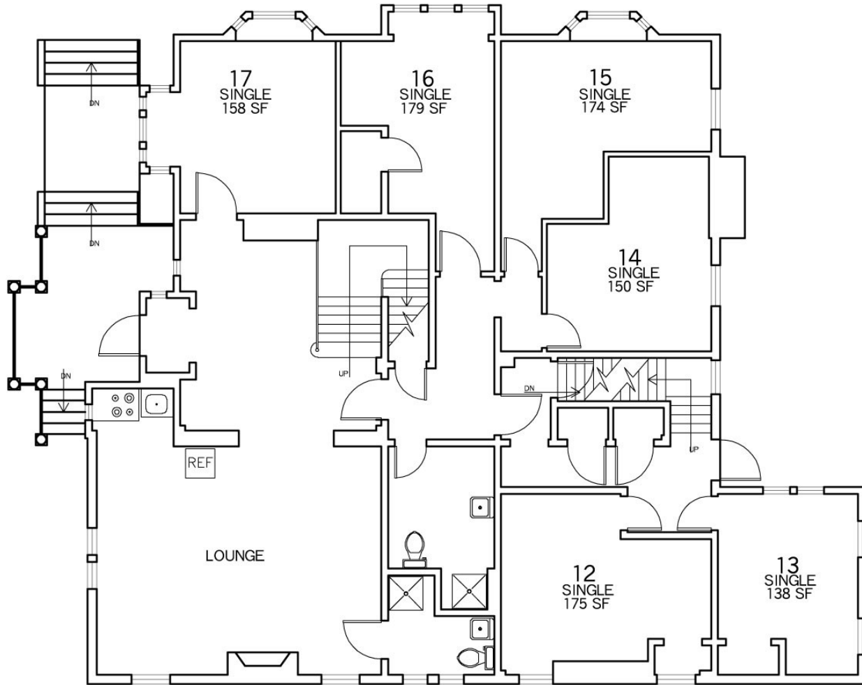
Nightengale House 54 Prospect Street First Floor Pan
